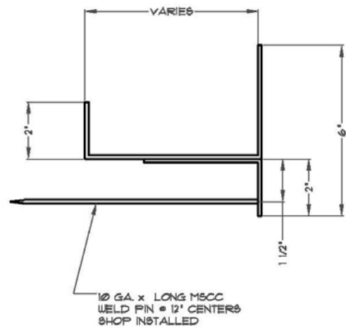
HILTI MODIFIED H-BAR
