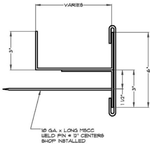
MODIFIED H-BAR & EXP. CLIP
